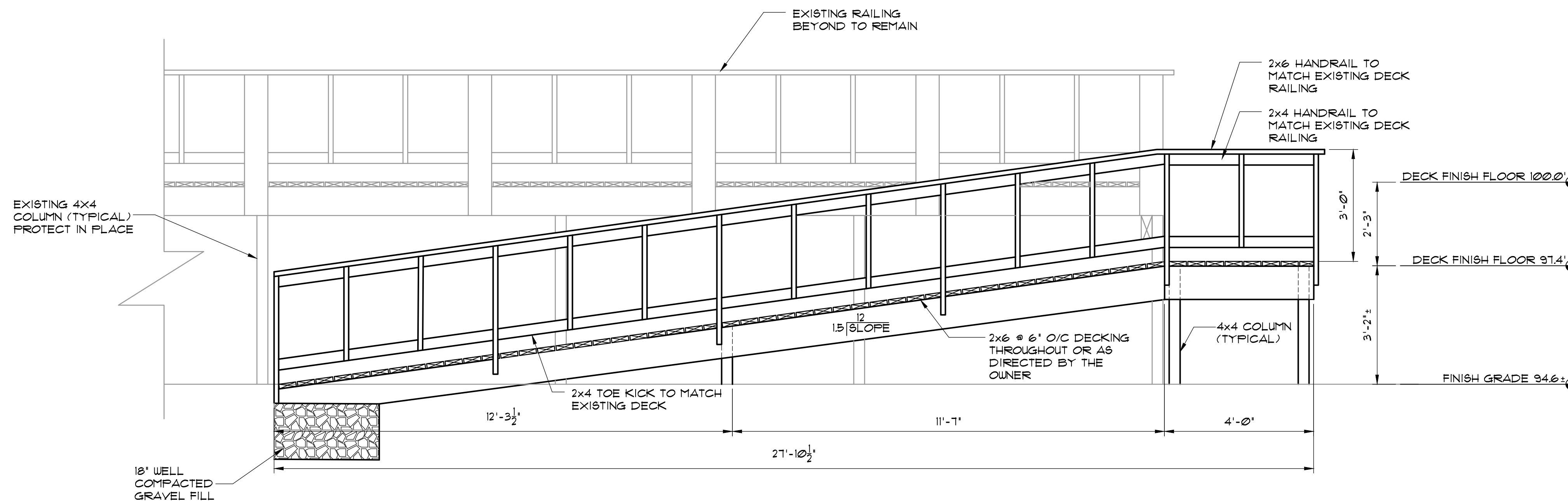
EAST RAMP ELEVATION SCALE: 1/2"=1'-0"
